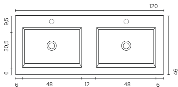
Akryl (B x D x H) 120 x 46 x 2 cm | 0 - 2 hanehuller
