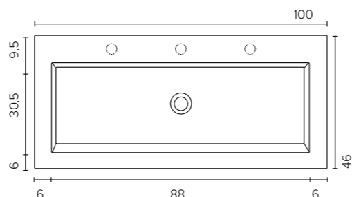
Akryl (B x D x H) 100 x 46 x 2 cm | 0 - 1 - 2 hanehuller
