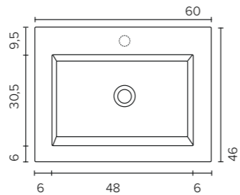
Akryl (B x D x H) 60 x 46 x 2 cm | 0 - 1 hanehuller
